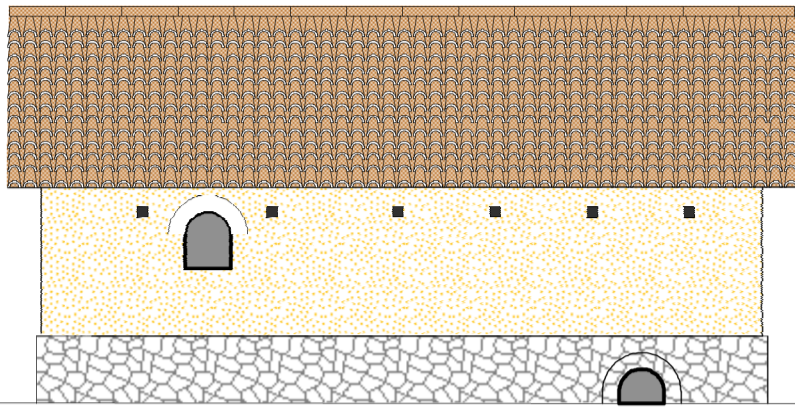
North-West Elevation
