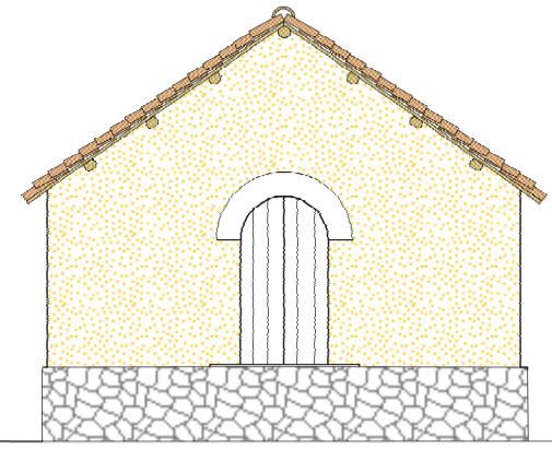
Front (North-East) Gable Elevation
